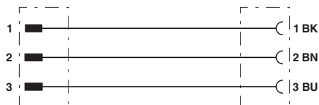
Contact assignment of 7/8" plugs/sockets
