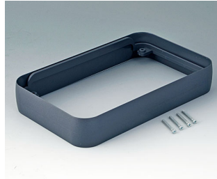
A9153018 Intermediate ring XL ABS (UL 94 HB) lava 3.78"x6.06"x1.02"
