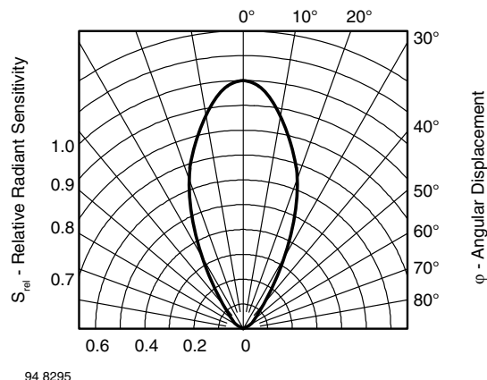
Fig. 10 - Relative Radiant Sensitivity vs. Angular Displacement
