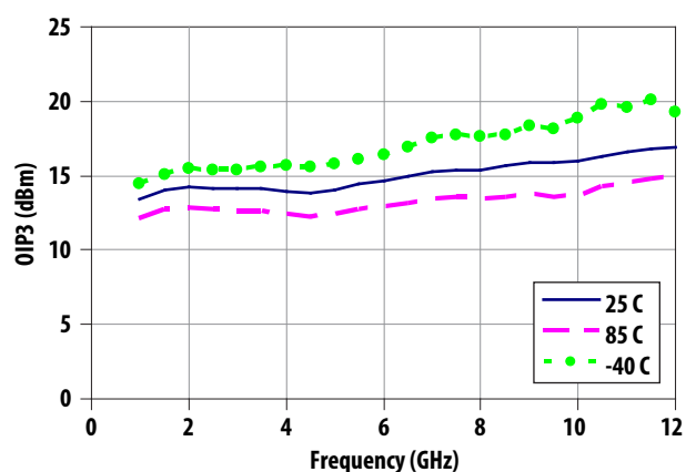
Figure 18. Output IP3 Over Temp [2,3]
