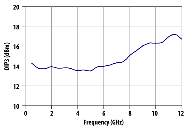
Figure 6. Output IP3 [1]
