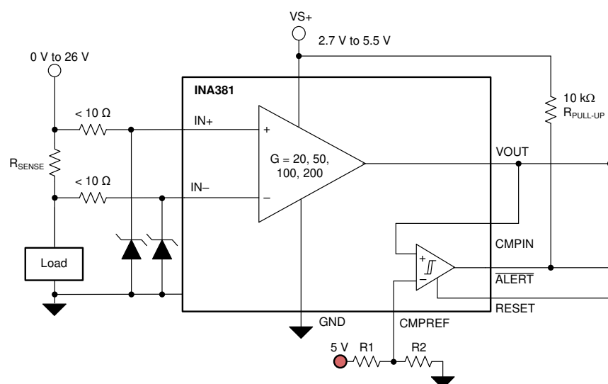
Figure 47. Transient Protection
