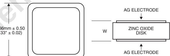
Uncoated Disk Part Number Suffix "KR"
