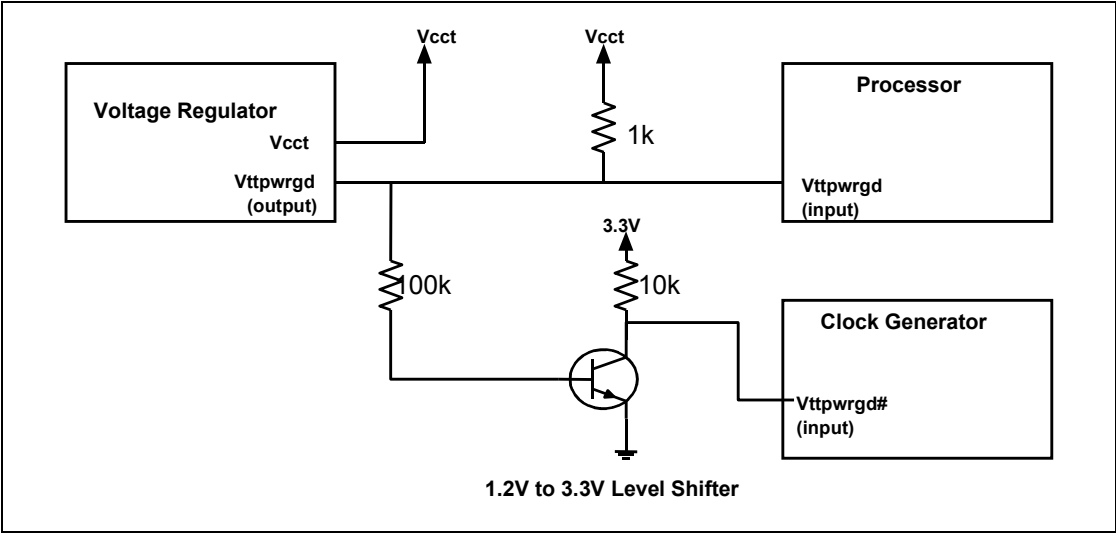
Figure 3. VTTWPRGD System-Level Connections
