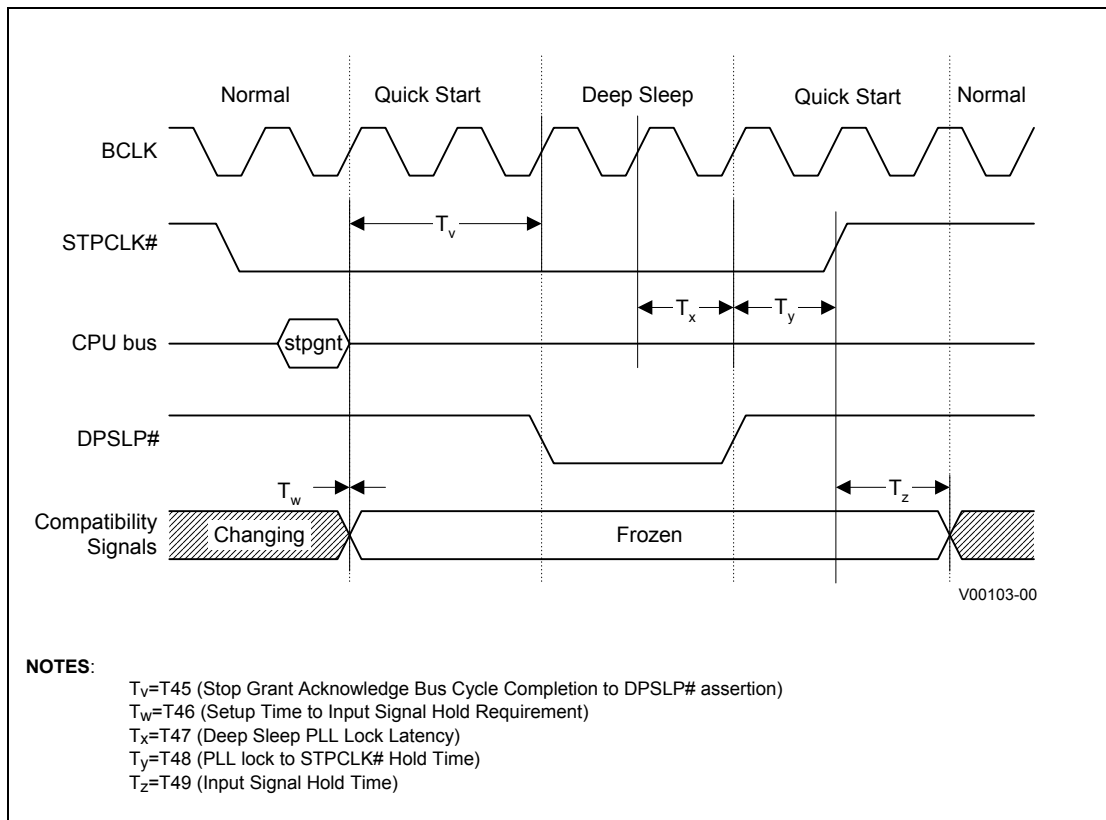
Figure 21. Quick Start/Deep Sleep Timing (DPSLP# Assertion Method)
