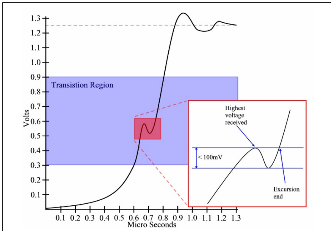
Figure 24. VTTPWRGD Noise Specification
