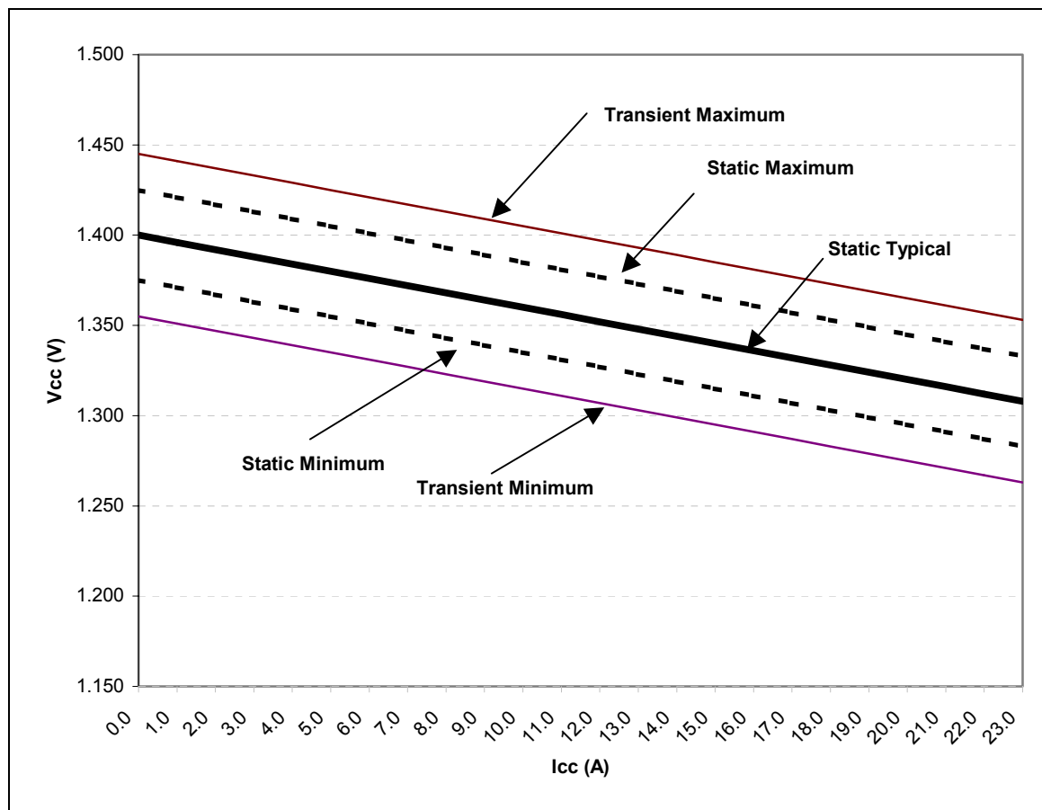
Figure 7. Illustration of V_{CC} Static and Transient Tolerances ( V_{ID} = 1.40\text{ V} )
