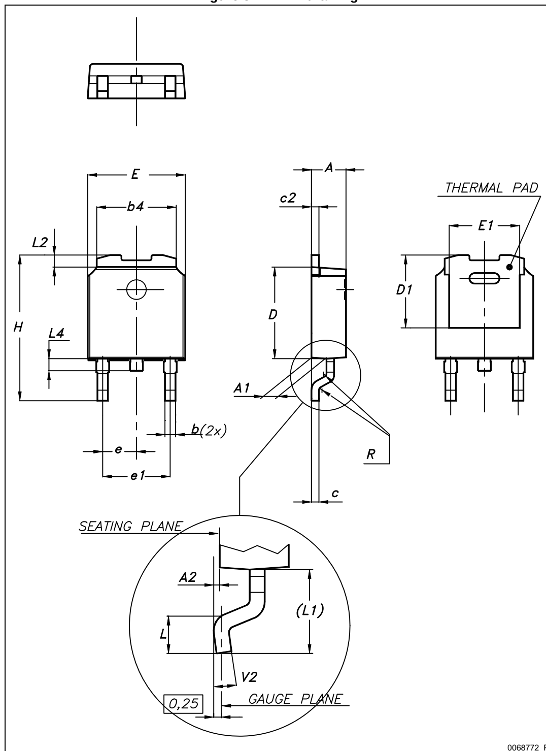
Figure 32. DPAK drawing
