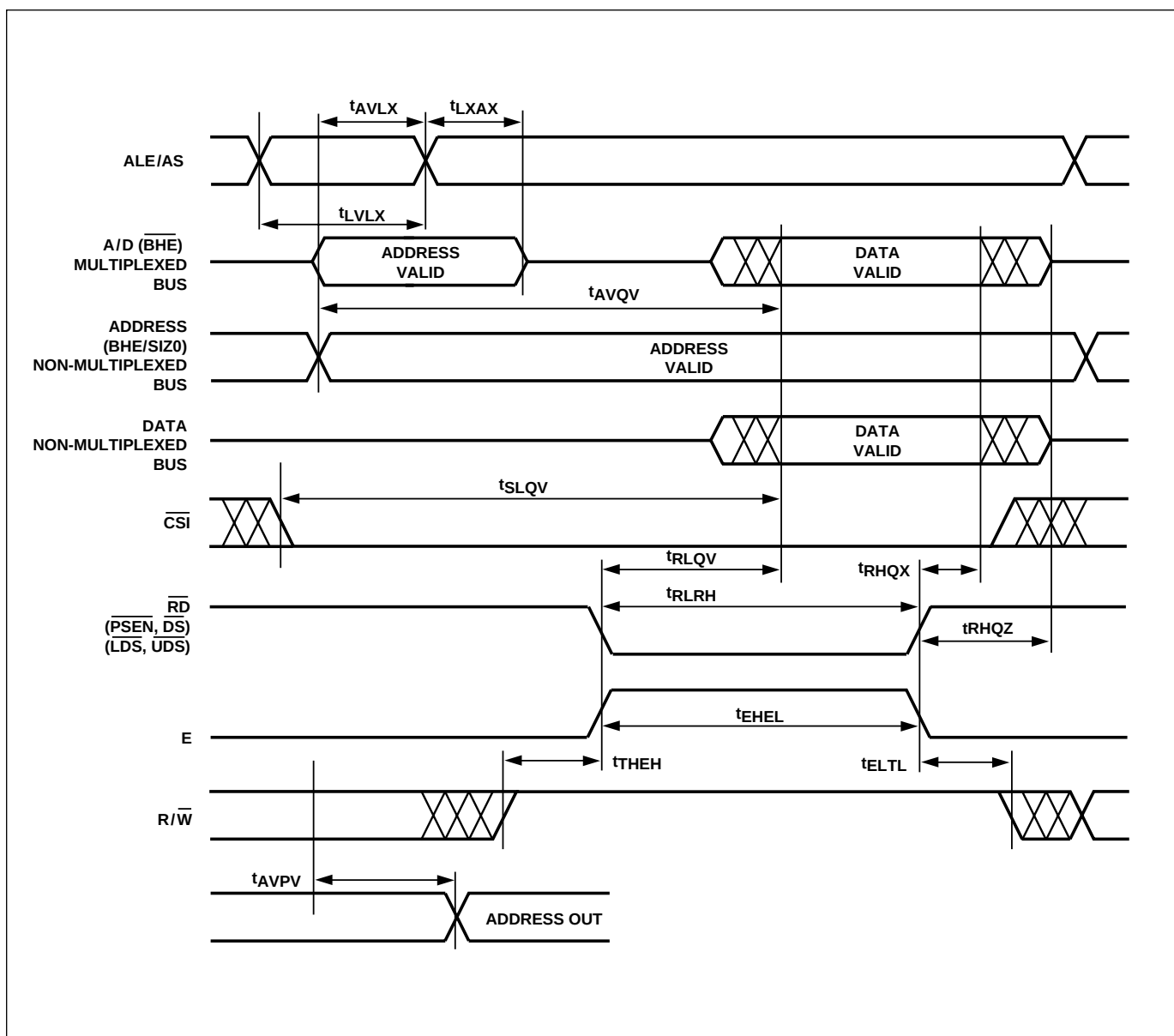
Figure 52. Read Timing
