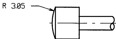
CONVEX RADIUS HEAD P1113CV2
