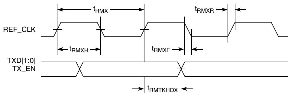
Figure 14. RMI Transmit AC Timing Diagram
