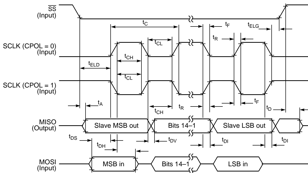
Figure 21. SPI Slave Timing (CPHA = 0)
