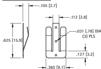
DWG. 2 MATERIAL: .010 (.25) Phosphor Bronze
