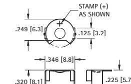
Thru Hole Mount
