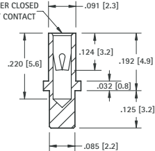
.032 (.81) - .046 (1.17) PIN - SOLDER MOUNT
