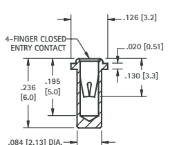
.032 (.81) - .046 (1.17) PIN - SOLDER MOUNT
