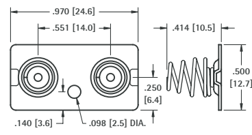
DUAL SPRING CONTACT
