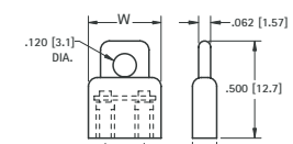
INSULATED SHORTING JACK
