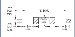
Pad Layout
