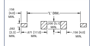
Pad Layout
