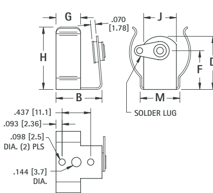
DWG. 2 Insulated Contact
