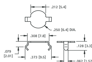
Mounting Detail
