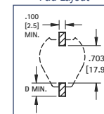
Pad Layout
