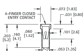
IC SOCKET CONTACTS FOR .015 (.38) - .025 (.64) LEADS - PRESS-FIT
