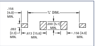
Pad Layout
