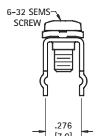
SNAP-IN PC MOUNT
