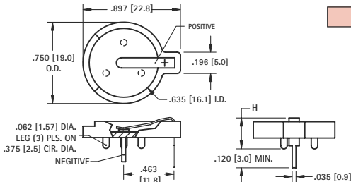
Mounting Detail
