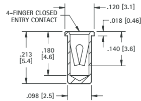
.048 (1.22) - .064 (1.63) PIN - SOLDER MOUNT
