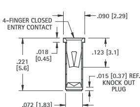
.032 (.81) - .046 (1.17) PIN - SOLDER MOUNT
