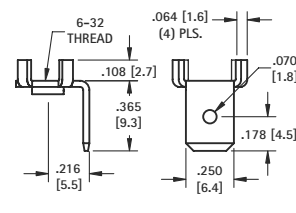
Mounting Detail
