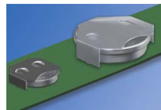
THRU HOLE MOUNT (THM)
