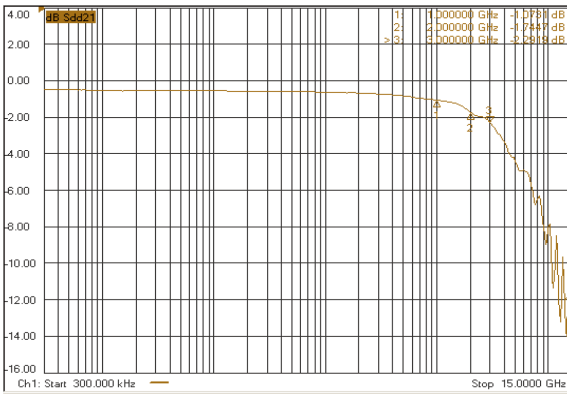
Insertion Loss
