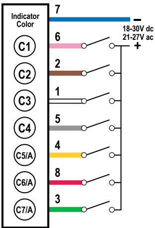
Sourcing (PNP) Input
