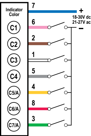
Sinking (NPN) Input
