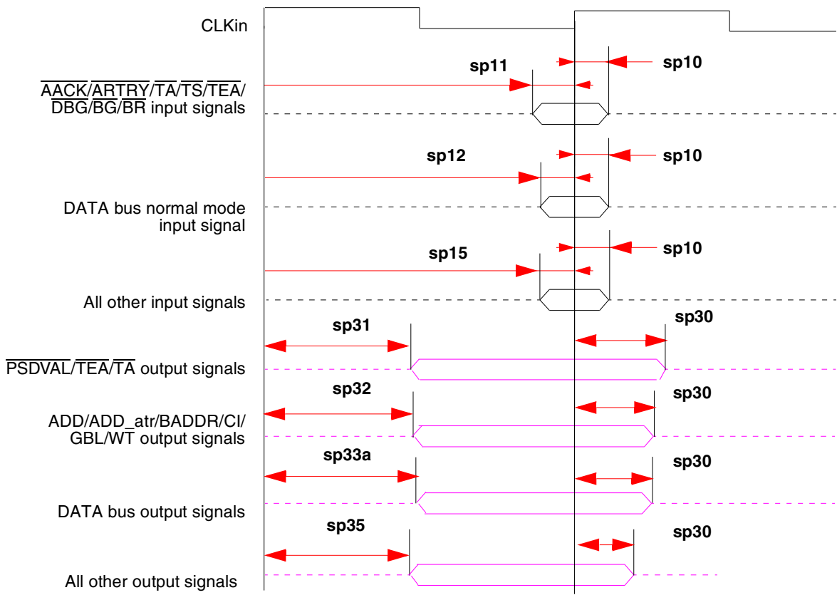
Figure 9. Bus Signals
