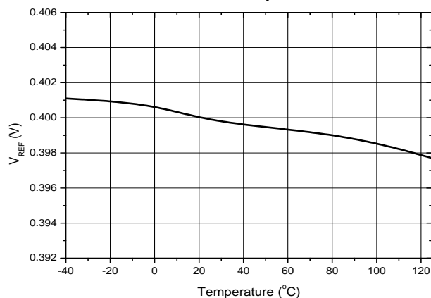
V_{REF} vs. Temperature
