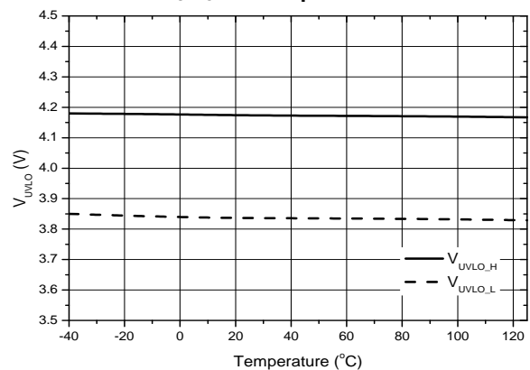
V_{UVLO} vs. Temperature
