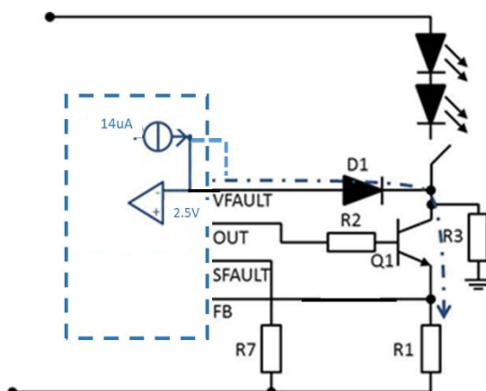
Figure 6. LED-Open Detection Using VFAULT
