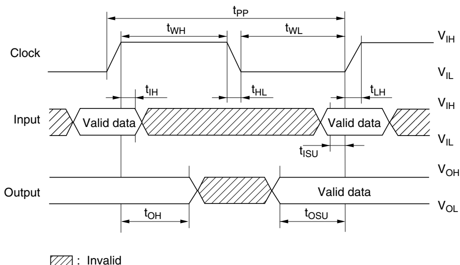
Timing Diagram of Data Input and Output
