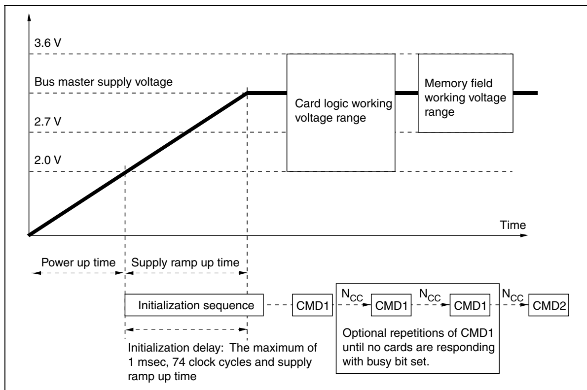
Power-up Diagram
