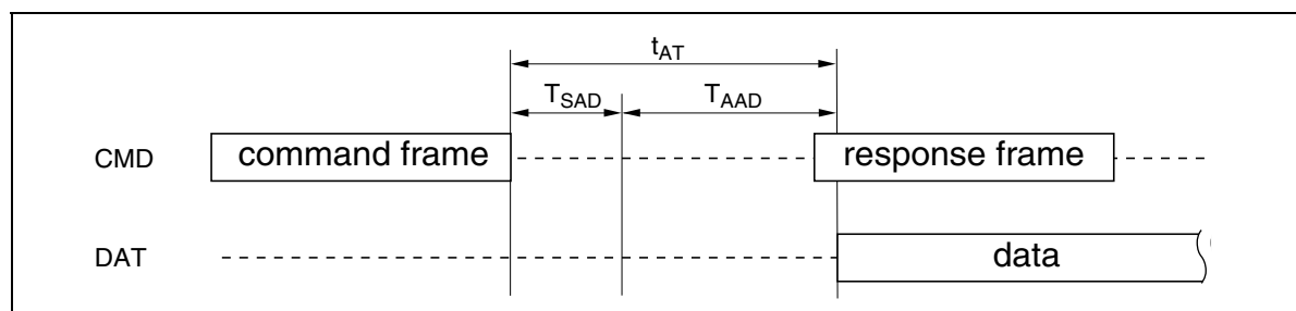
Access Time
