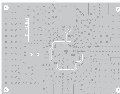
Layer 4: Solid Ground Plane
