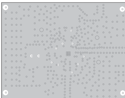
Layer 3: Power Plane
