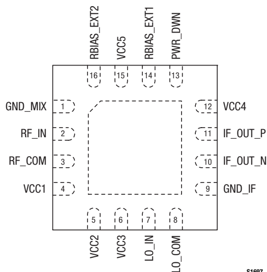
Figure 2. SKY73049-350LF Pinout – 16-Pin QFN (Top View)
