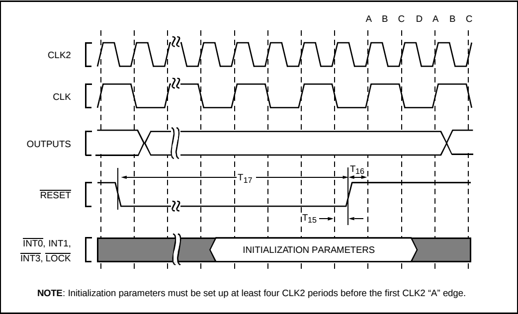
Figure 13. \overline{RESET} Signal Timing
