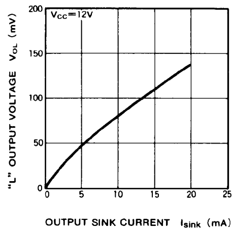
"L" OUTPUT VOLTAGE VS. OUTPUT SINK CURRENT
