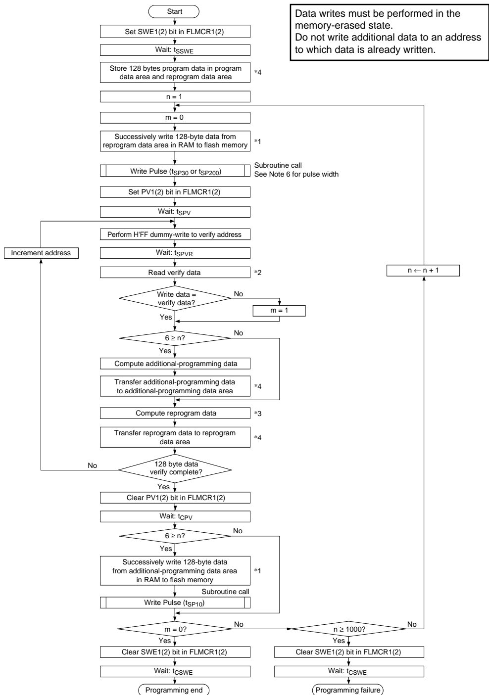
Figure 22.13 Program/Program-Verify Flowchart (1)
