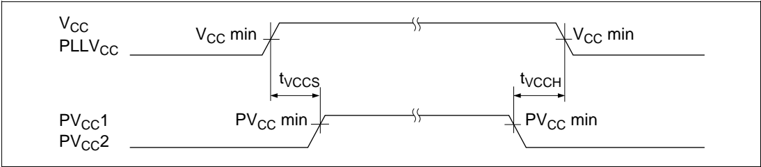
Figure 25.1 Power-On/Off Timing
