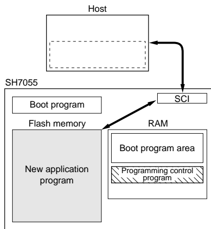
Figure 22.3 Boot Mode
