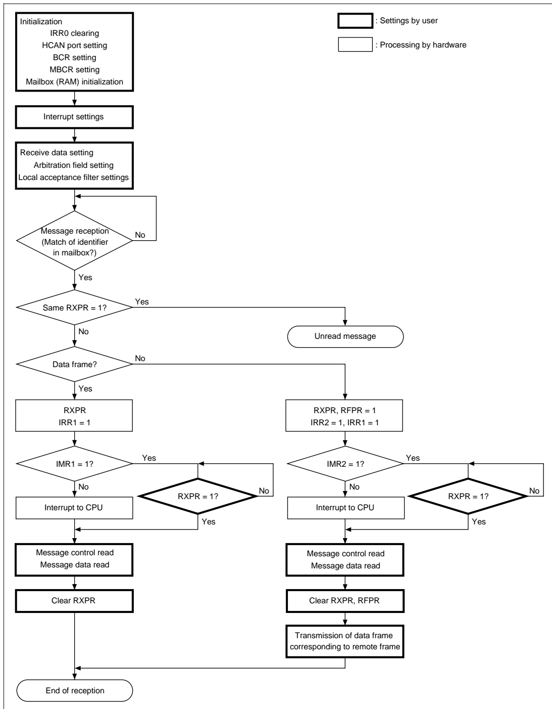
Figure 16.11 Reception Flowchart
