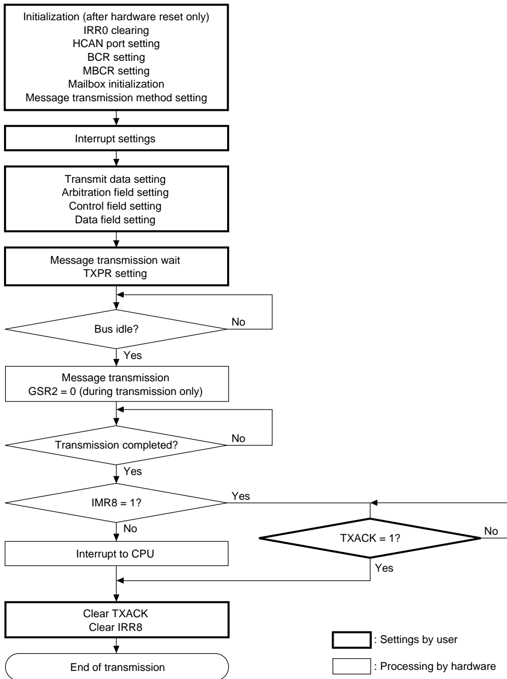
Figure 16.9 Transmission Flowchart
