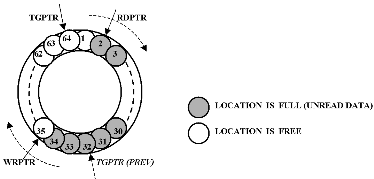
Figure 35. Circular Buffer
