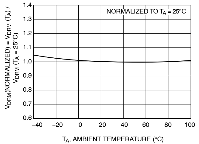
Figure 6. Normalized Off-State Output Terminal Voltage vs. Ambient Temperature
