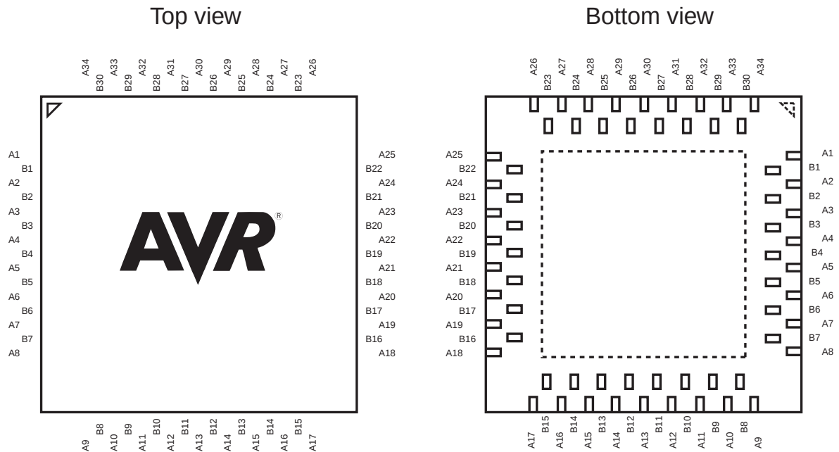
Figure 2-2. DRQFN pinout for ATxmega128B3
