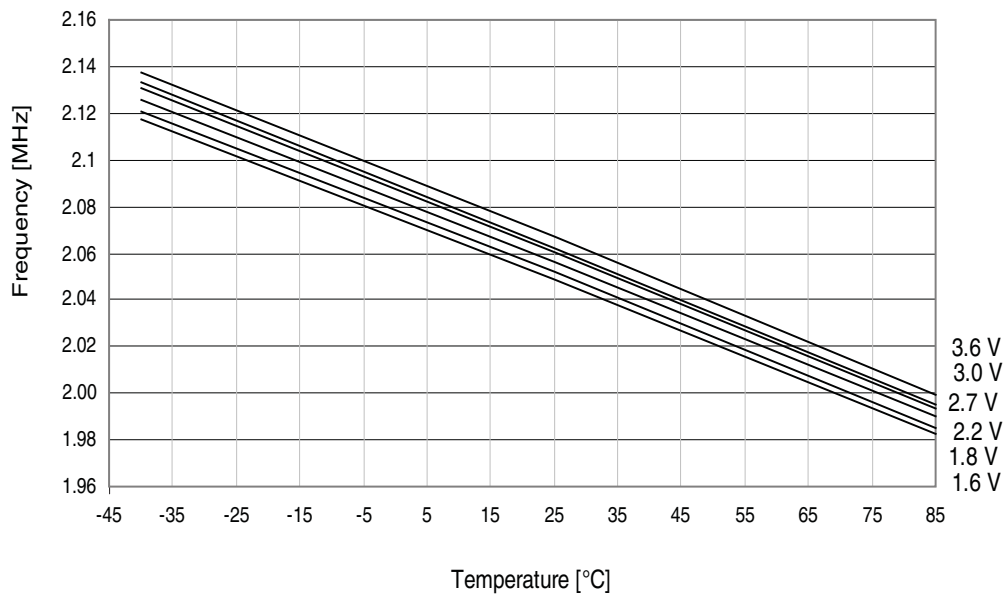
Figure 37-62. 2MHz internal oscillator frequency vs. temperature.
