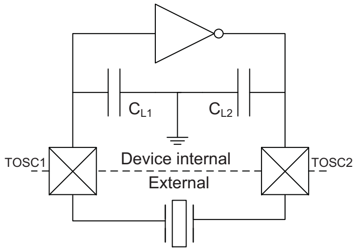
Figure 36-4. TOSC input capacitance
