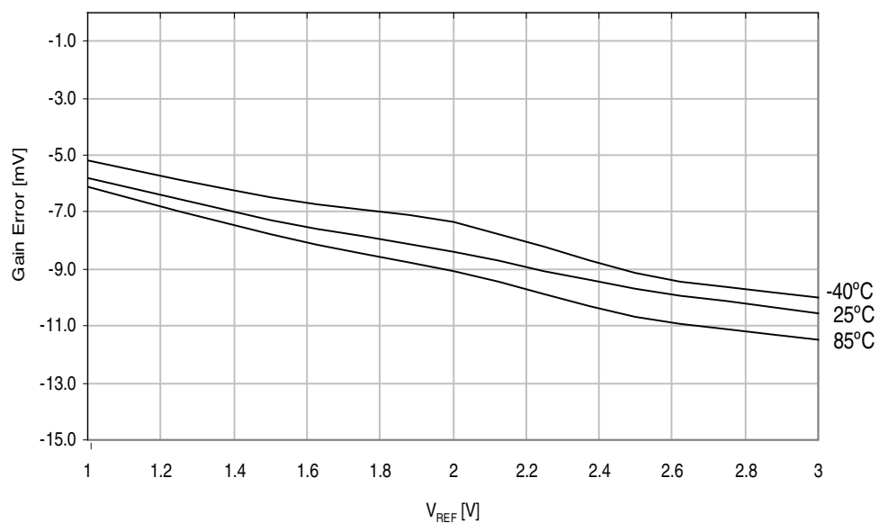
Figure 37-32. ADC Gain Error vs. V_{REF} .
