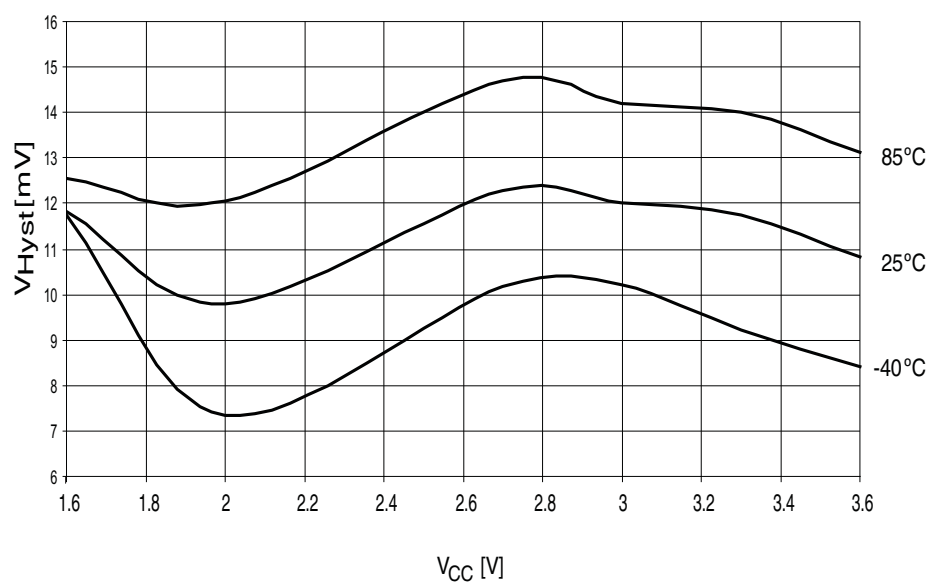
Figure 37-38. Analog comparator hysteresis vs. V_{CC} . High-speed mode, small hysteresis.
