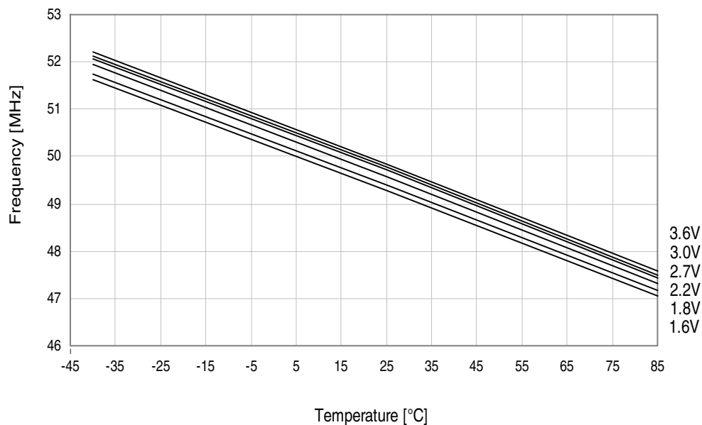
Figure 37-72. 48MHz internal oscillator frequency vs. temperature.
