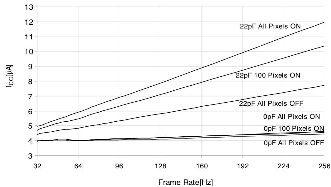
Figure 37-77. I_{CC} vs. Frame Rate 32Hz Low Power Frame Rate from 32.768KHz TOSC, w/ and w/o pixel load, V_{CC} = 3.0V , T = 25^{\circ}C
