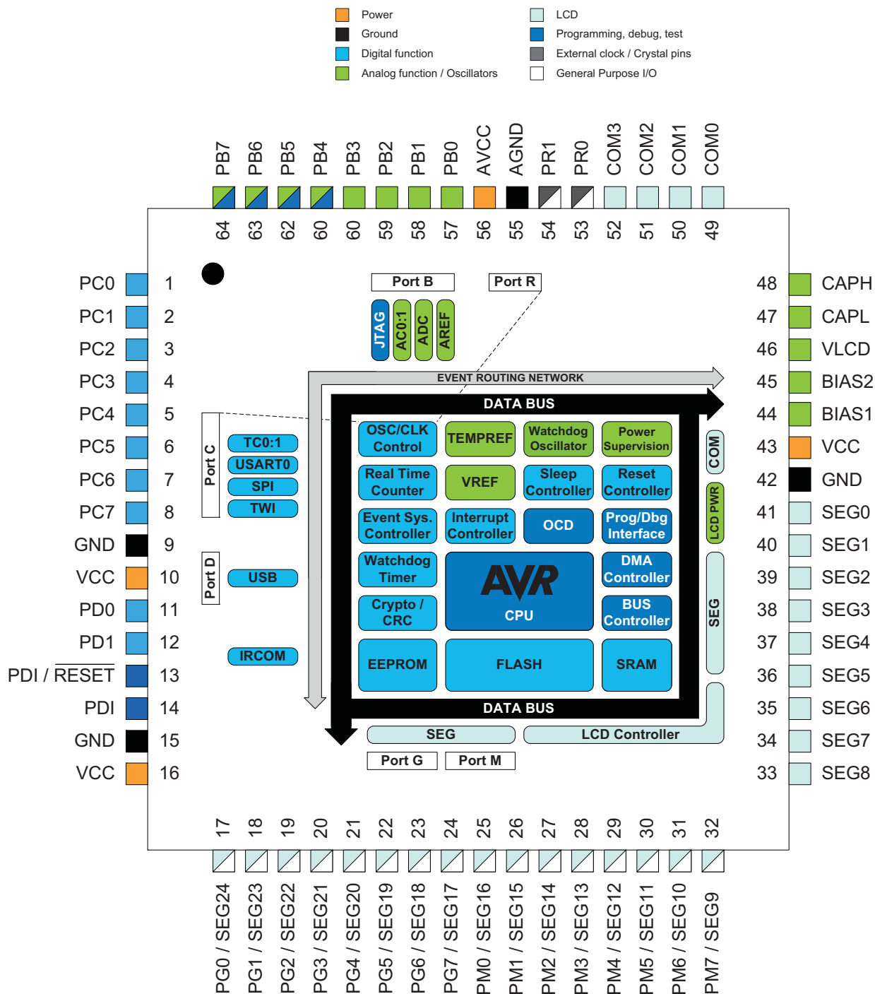
Figure 2-1. Block diagram and TQFP/QFN pinout
