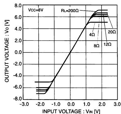
Fig.18 Load fluctuation I/O characteristic ch2 (Ta=85°C)
