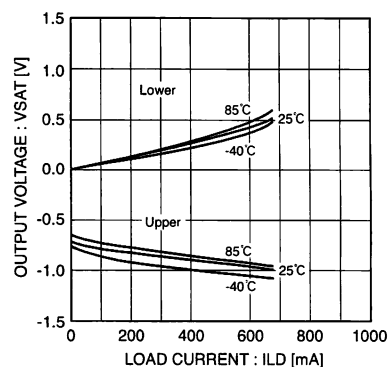
Fig.30 Load fluctuation temperature characteristic (Loading driver) ( V_{cc} = 8\text{V} )
