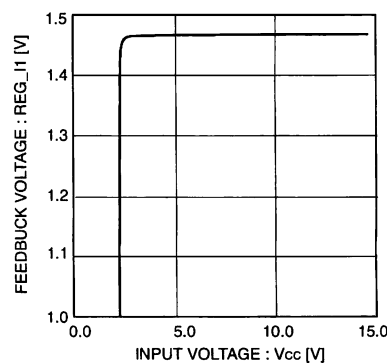
Fig.24 Regulator1 terminal supply voltage characteristic (Ta=85°C)
