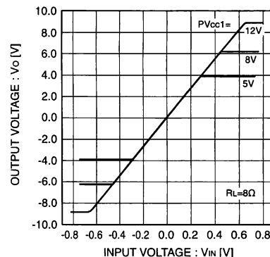
Fig.9 Supply fluctuation I/O characteristic (Ta = 85°C)
