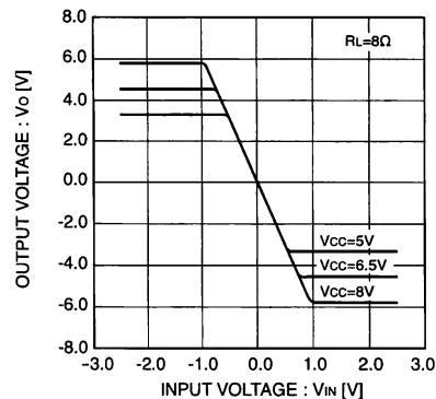
Fig.3 Supply fluctuation I/O characteristic (Ta = 85°C)
