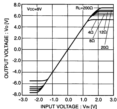
Fig.15 Load fluctuation I/O characteristic ch1 (Ta=85°C)
