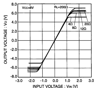
Fig.21 Load fluctuation I/O characteristic ch3 (Ta=85°C)
