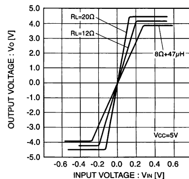
Fig.12 Load fluctuation I/O characteristic (Ta = 85°C)
