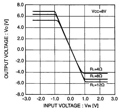
Fig.6 Load fluctuation I/O characteristic (Ta = 85°C)
