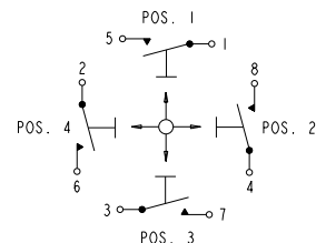
(C) SPST-NO 4 WAY SCHEMATIC
