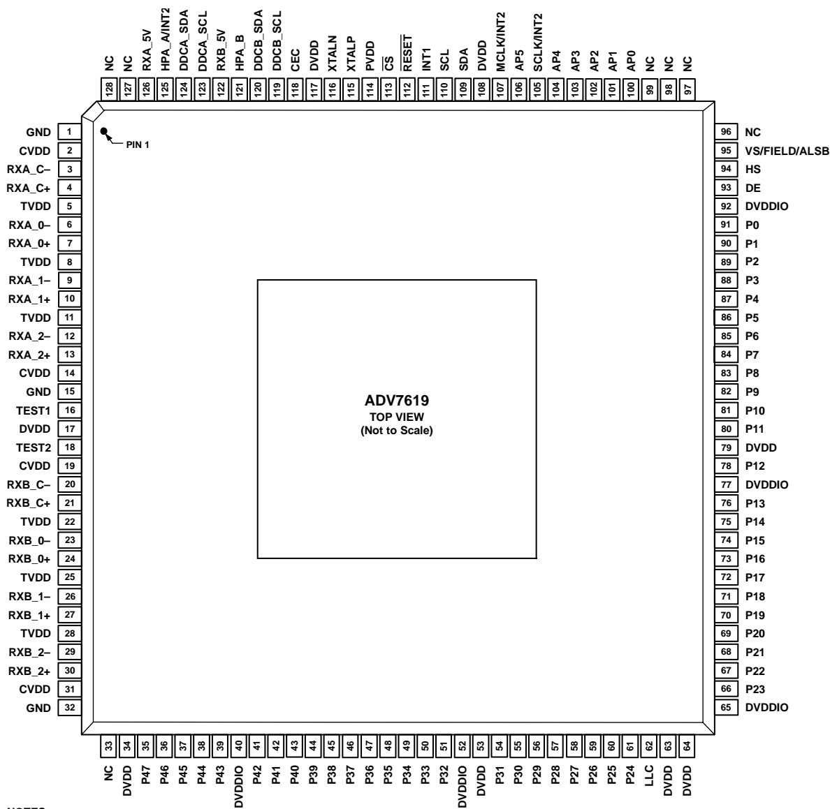
Figure 6. Pin Configuration
