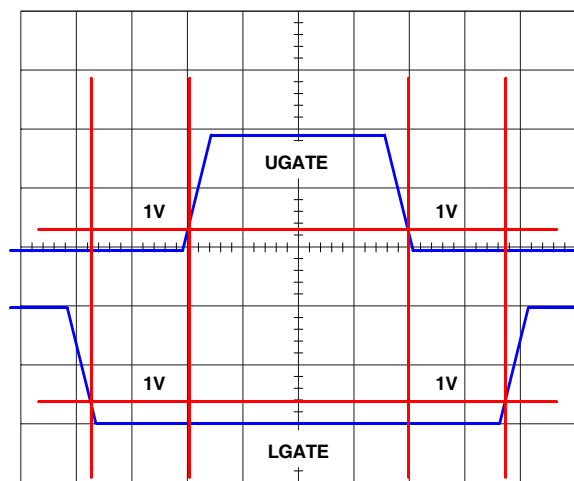
FIGURE 19. GATE DRIVE ADAPTIVE SHOOT-THROUGH PROTECTION
