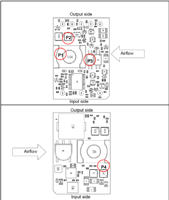
Open frame
