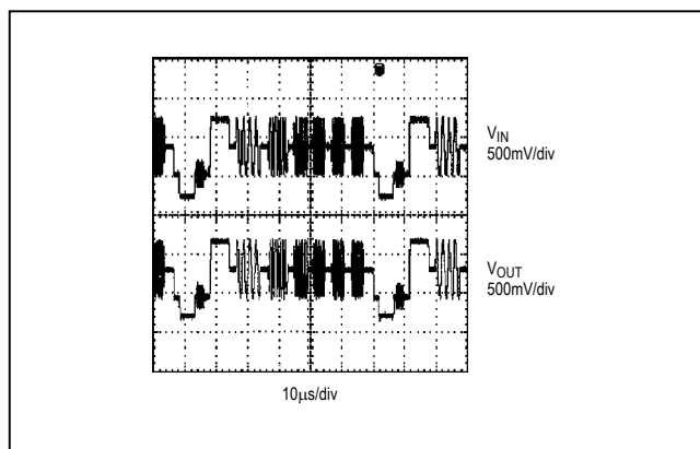
Figure 3. Multiburst Response
