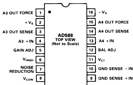
D Package
