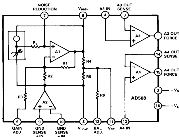
D Package
