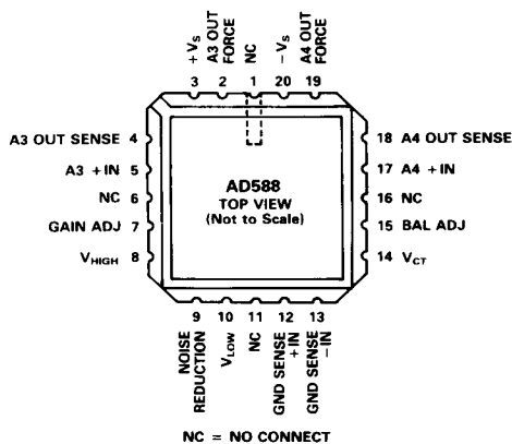
E Package
