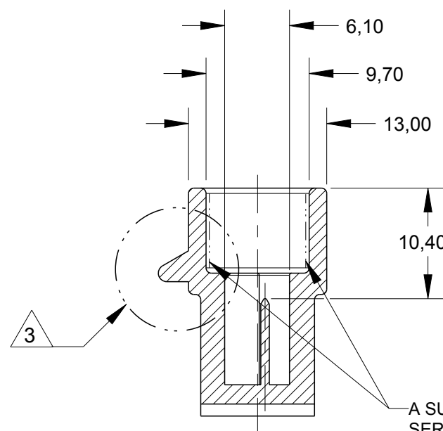
SECTION B-B
