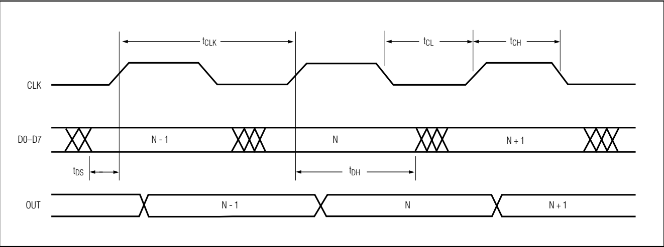
Figure 4. Timing Diagram
