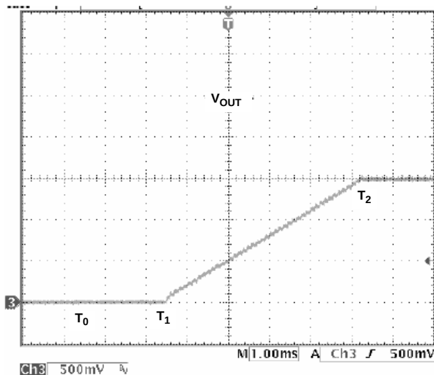
FIGURE 20. NORMAL START-UP
