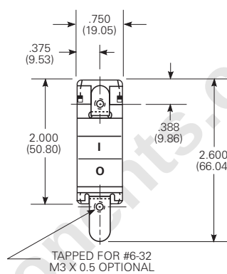
VDE Rocker Marking
