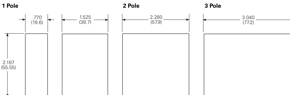
Panel Mounting Cutout
