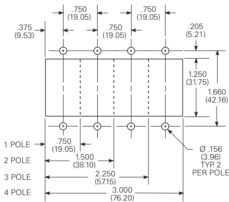
Panel Mounting Cutout
