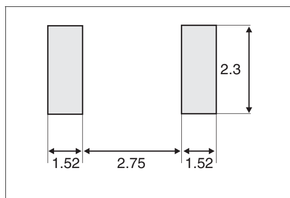
Figure 19: SMB Foot Print Dimensions (in millimeters)
