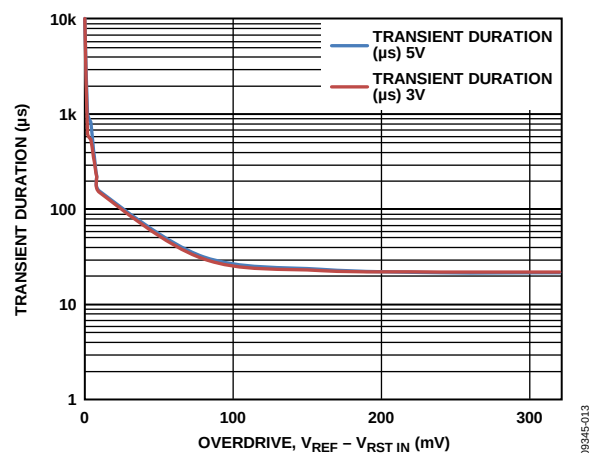
Figure 13. Maximum Transient Duration vs. RST INx ( V_{TH} = 0.4 V) Threshold Overdrive
