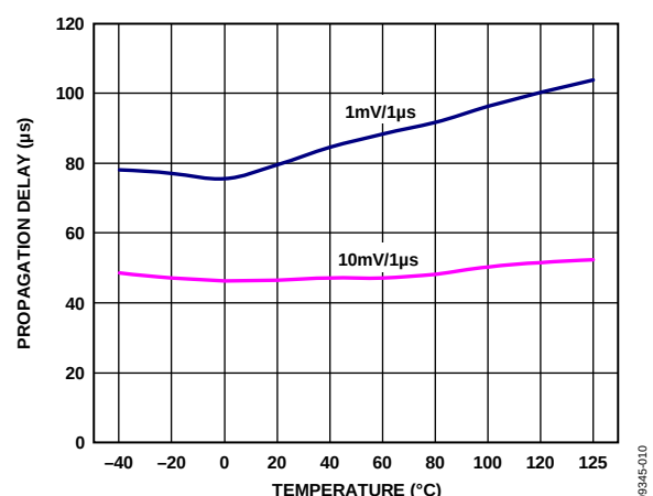
Figure 10. RST IN ( V_{TH} = 1.23\text{ V} ) Falling Propagation Delay vs. Temperature
