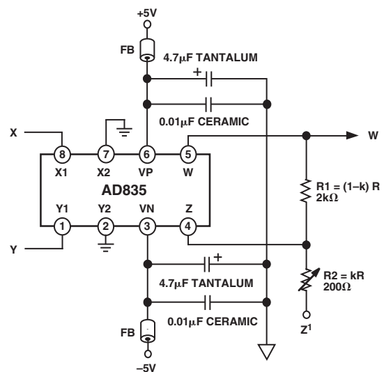
Figure 2. Multiplier Connections
