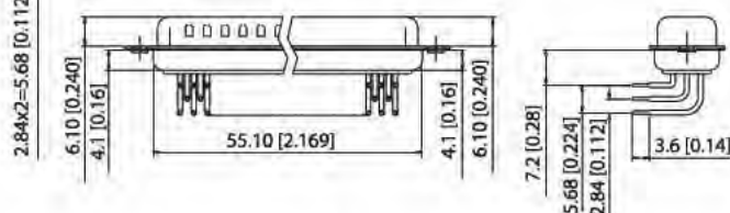
50 Positions Machined Pin (W/O Rear Cover)
