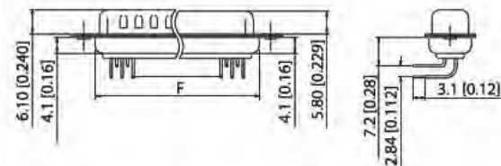
7.2mm[0.28"] Footprint Machined Pin (W/O Rear Cover)
