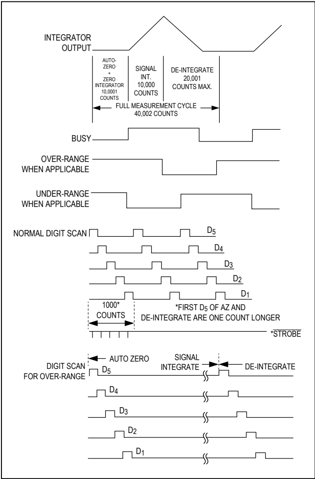
Figure 4. Timing Diagram
