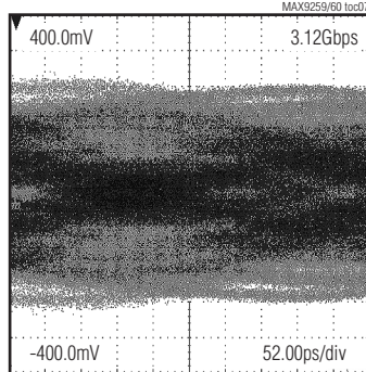
SERIAL LINK SWITCHING PATTERN WITHOUT PREEMPHASIS (PARALLEL BIT RATE = 104MHz, 10m STP CABLE)
