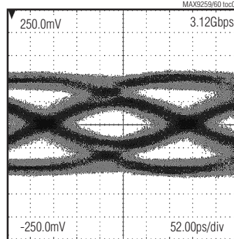
SERIAL LINK SWITCHING PATTERN WITH 14dB PREEMPHASIS (PARALLEL BIT RATE = 104MHz, 10m STP CABLE)
