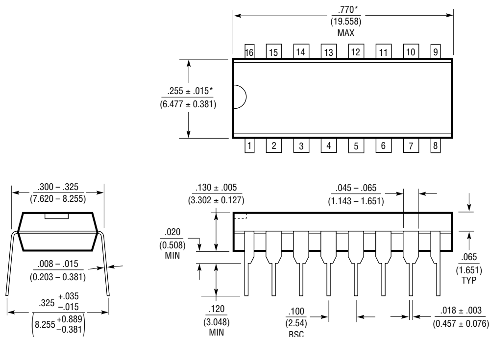
N Package 16-Lead PDIP (Narrow .300 Inch) (Reference LTC DWG # 05-08-1510)
