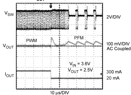
Mode Change by Load Transients V_{OUT} = 2.5V (PWM to PFM)
