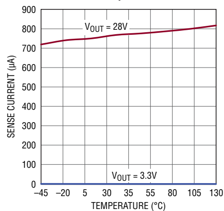
Buck SENSE Pins Total Input Current vs Temperature
