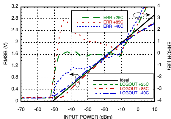
RMSB & Error vs. Pin @ 3900 MHz [1]
