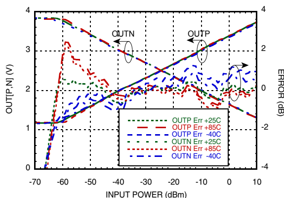
OUT [P,N] & Error vs. Pin @ 900 MHz [1][2]
