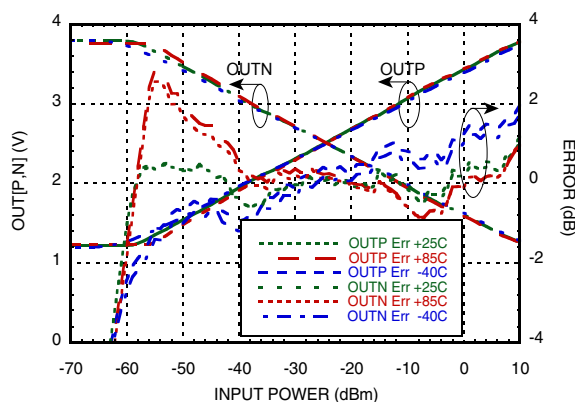
OUT [P,N] & Error vs. Pin @ 2200 MHz [1][2]
