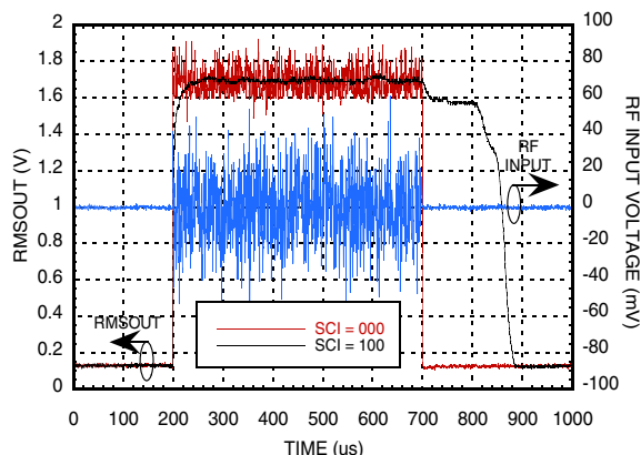
Residual Ripple for 0.9 GHz WCDMA-4TM @ SCI = 100
