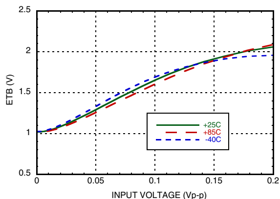
ETB vs. Pin with CW @ 900 MHz
