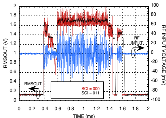
Residual Ripple for 0.9 GHz LTE Downlink @ SCI = 011
