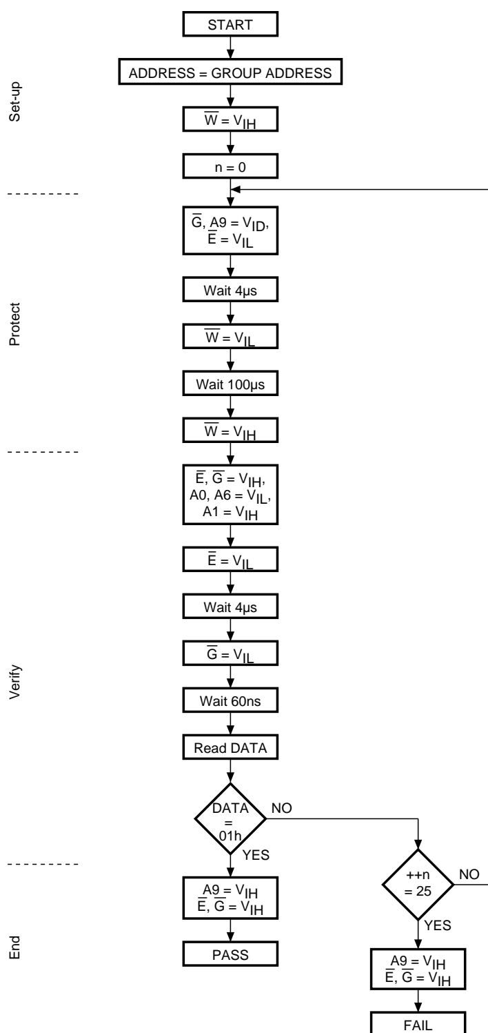
Figure 14. Programmer Equipment Group Protect Flowchart
