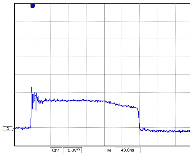
Figure 3 – Clamping Characteristics when device subjected to an 8 KV ESD pulse.
