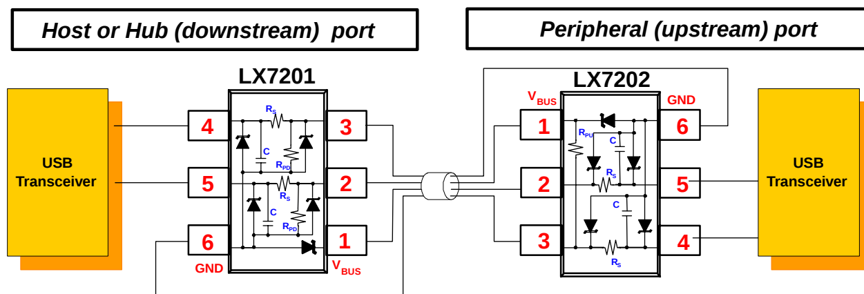
Figure 1 – Typical Application
