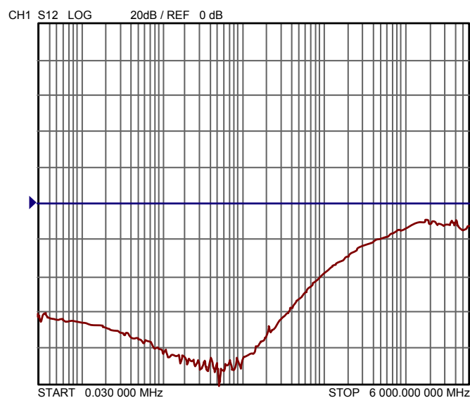
Figure 5 – Analog Crosstalk between the two datalines D- and D+
