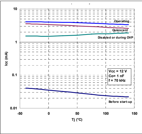
Figure 5. IC consumption vs T_J
