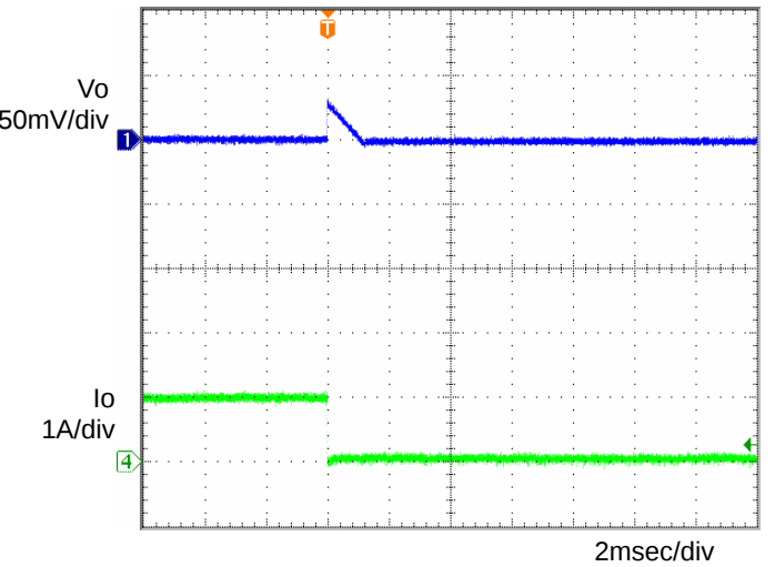
Fig.6 Transient Response (1.0→0A) Co=1 \mu F, Ta=-40°C
