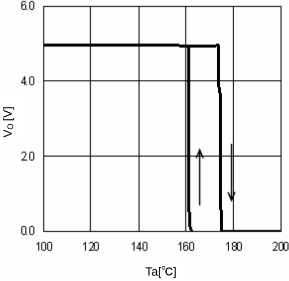
Fig.28 TSD ( I_o=0mA )
