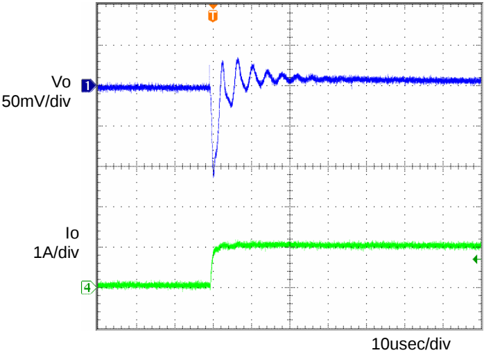
Fig.4 Transient Response (0→1.0A) Co=1 \mu F, Ta=25°C
